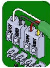
DETAIL H 4-WIRE CONNECTION
